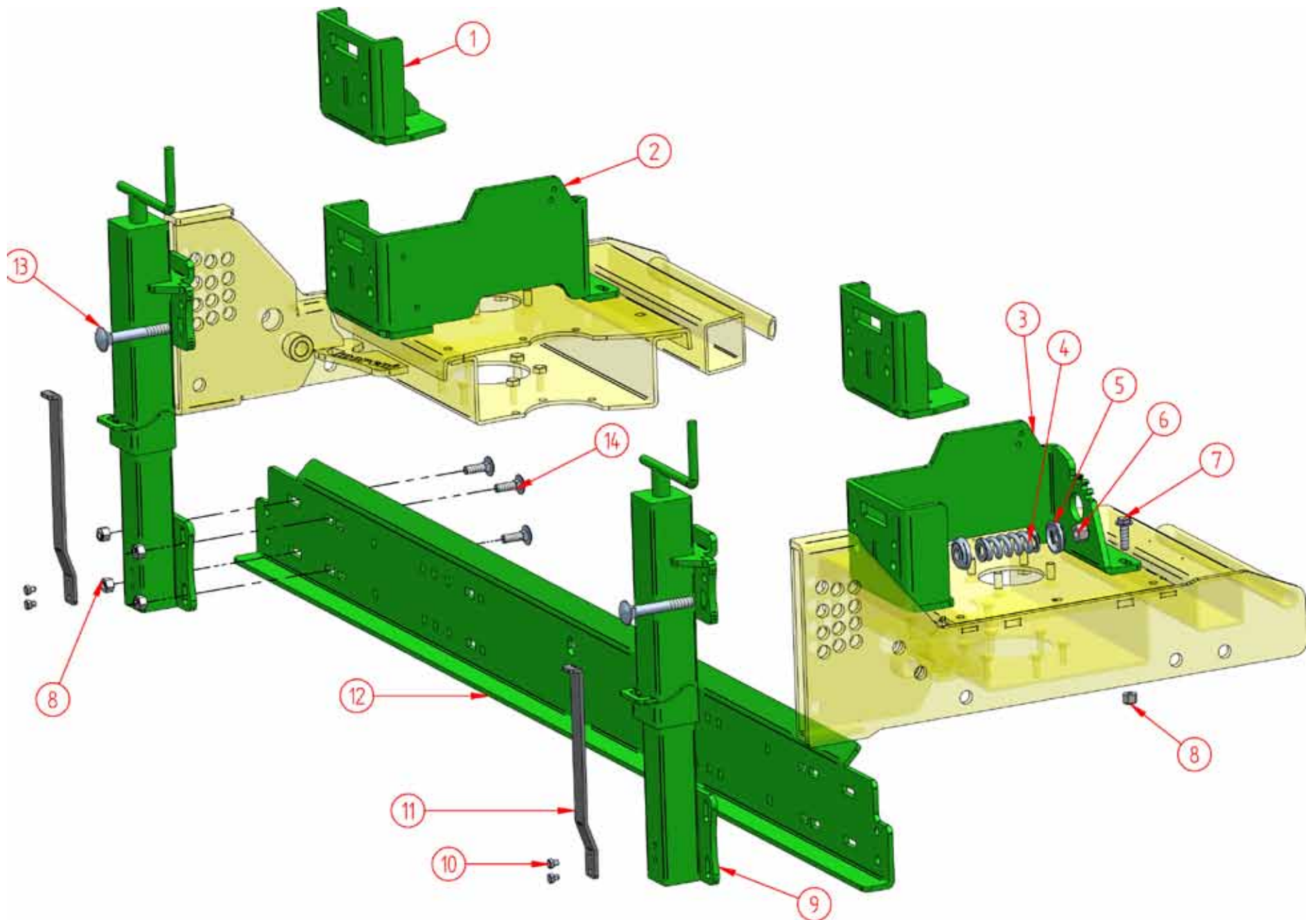
BARRA POSTER. ERPICI FISSI - BAR HANDLE'S CONNECTION
